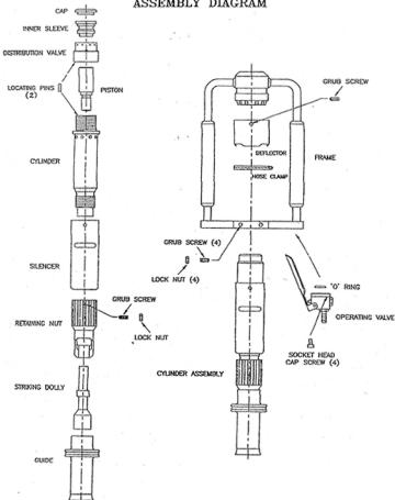
CYLINDER ASSEMBLY
